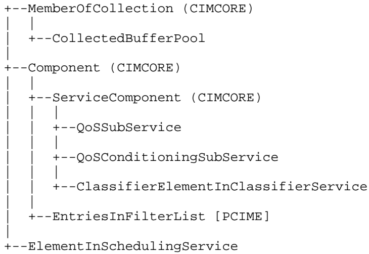
Figure 11. Aggregation Class Inheritance Hierarchy
