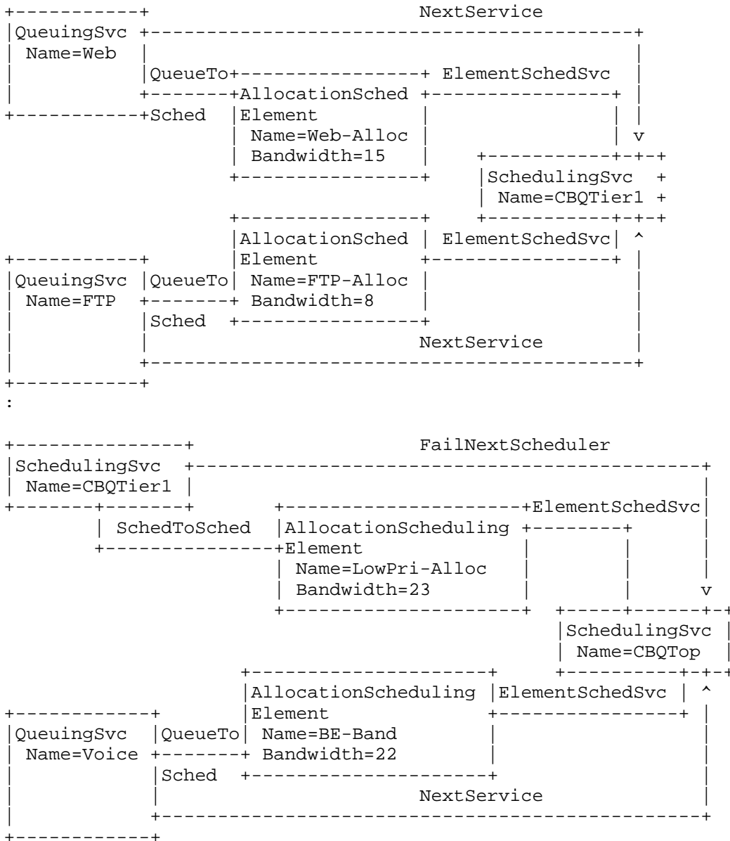
Figure 8. Example 4: Hierarchical CBQ Scheduler
